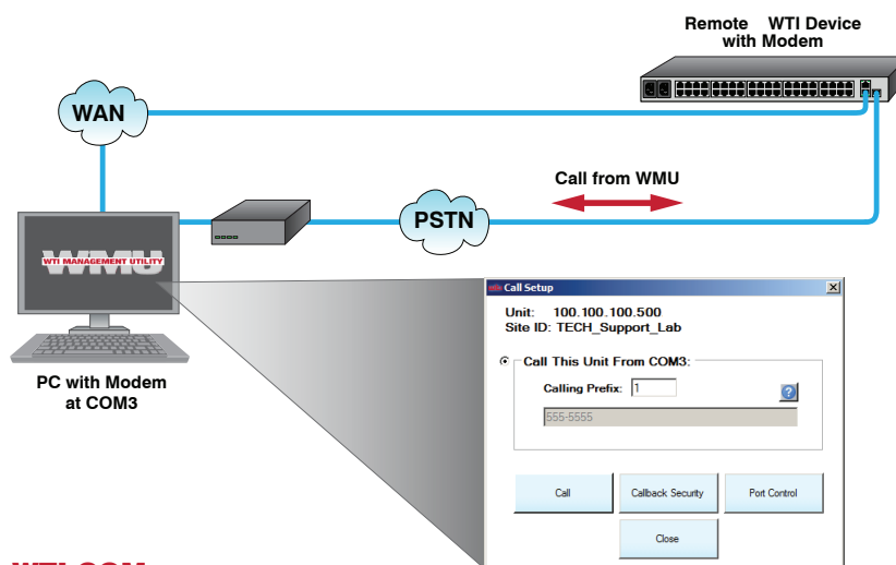
Figure 1: Call This Unit From COM Port - Example
