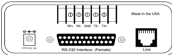
Figure 3. Rear view of Model 1080A Series - AC Power
