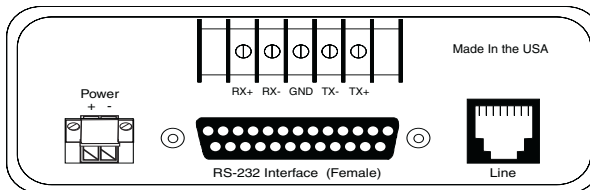
Figure 4. Rear view of Model 1080A Series - DC Power
